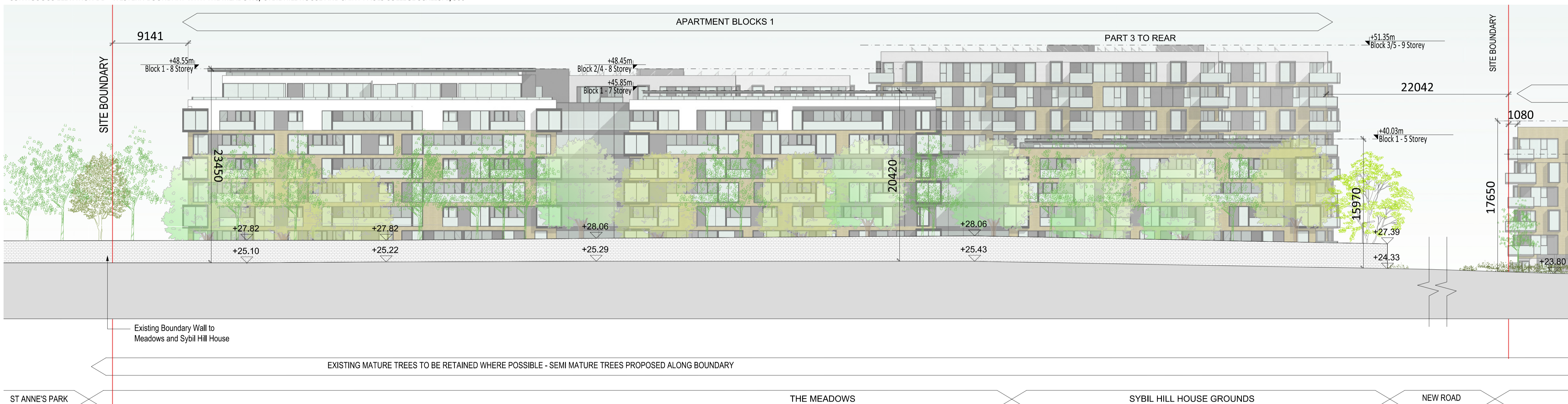
CONTIGUOUS ELEVATION DD (PART 1) - WESTERN BOUNDARY WITH THE MEADOWS/ SYBIL HILL HOUSE AND SAINT PAULS COLLEGE SCALES: 1/250
